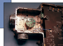
NASA's Global Hawk carrying a synthetic aperture radar payload (inset) on a fully unmanned aerial recon mission uses internal DSP-1750 gyros from KVH to maintain focused and stable imagery.
