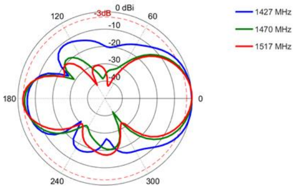
Elevation: 1427 – 1517 MHz Elevation: 1710 – 2170 MHz
