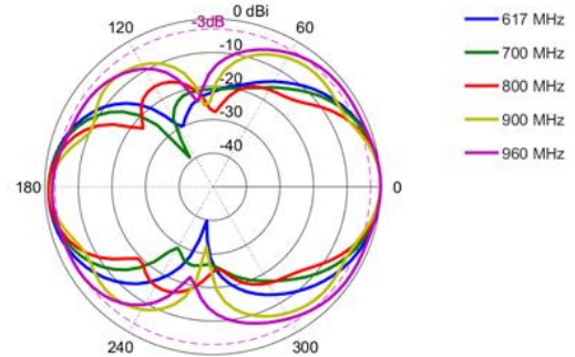
Azimuth: 3400 – 3800 MHz Elevation: 617 – 960 MHz
