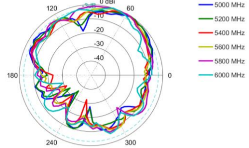
Elevation: 5000 – 6000 MHz
