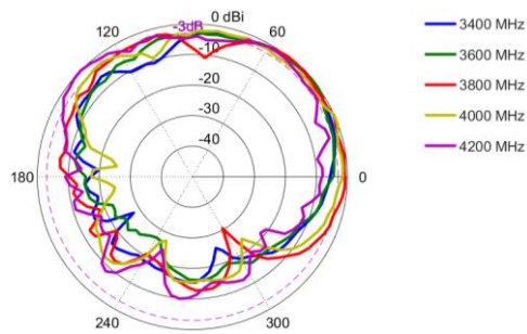
Elevation: 3400 – 4200 MHz
